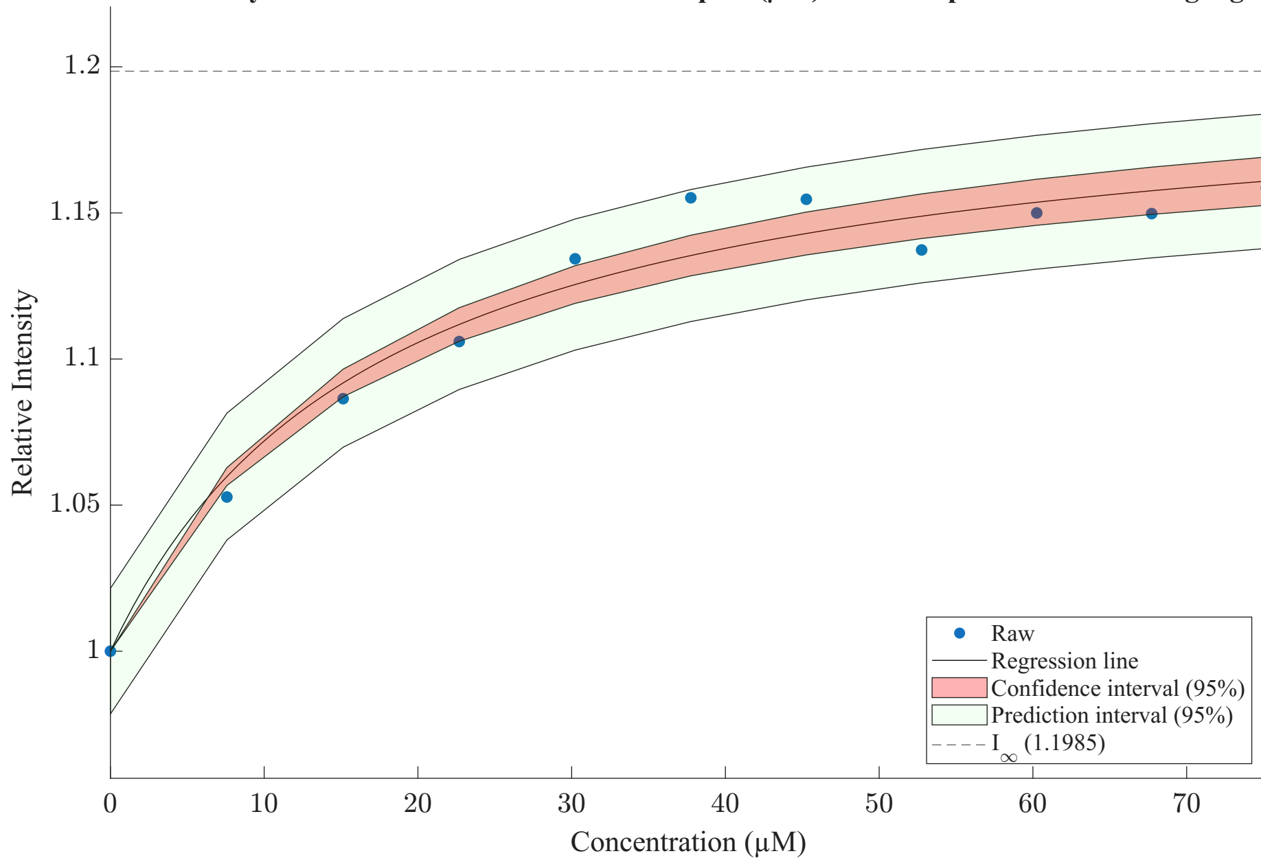
Relative intensity as a function of concentration of lipids (μM) for a6r rep1 - Statistics fitting algorithm
